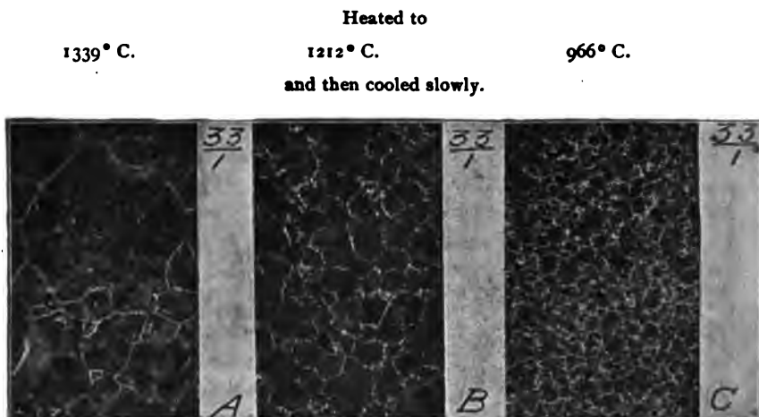
Fig. 76a. Influence of the Highest Temperature Reached ( T_{max} ) on the Size of the Grain of Slowly Cooled Steel. 33 Diameters.
